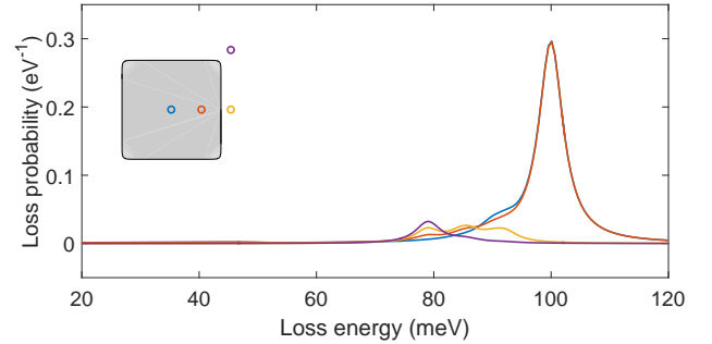
FIG. 4: Loss probability for a single 50 nm MgO nanocube and for an electron beam with a kinetic energy of 60 keV. The results are computed for various electron beam positions shown in the inset using a local dielectric description and the simulation software of Refs. 24,27. We use the dielectric function of Eq. (13) with values of \omega_{\text{TO}} = 50 meV, \omega_{\text{LO}} = 100 meV, \eta = 5 meV, and \epsilon_{\infty} = 3 representative for MgO (Ref. 28). The peak at 100 meV is due to bulk losses to LO phonons, whereas the peaks at lower energies are due to surface phonon polariton excitations localized at the corners, edges, and faces of the cube. Note that for the intersecting geometries (red and blue lines) there are no excitations present below 60 meV.
