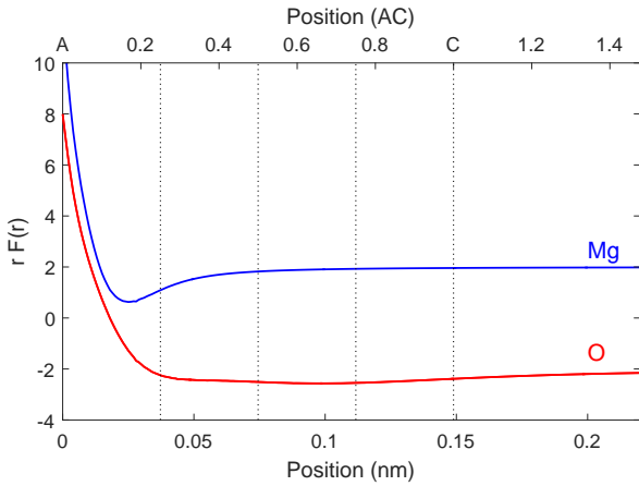
FIG. 2: Force F(r) acting on a single ion as the impact parameter \mathbf{R}_0 is varied along the direction AC, indicated in Fig. 1, for realistic charge distribution of ions (for details see text). The force exerted by the electron beam has an approximate 1/r -dependence 17 , in the figure we plot rF(r) rather than the force itself. For small distances the force approaches the atomic numbers of 12e and 8e for Mg and O, respectively, whereas for larger distances it approaches the effective ion charges of \pm 2e .
